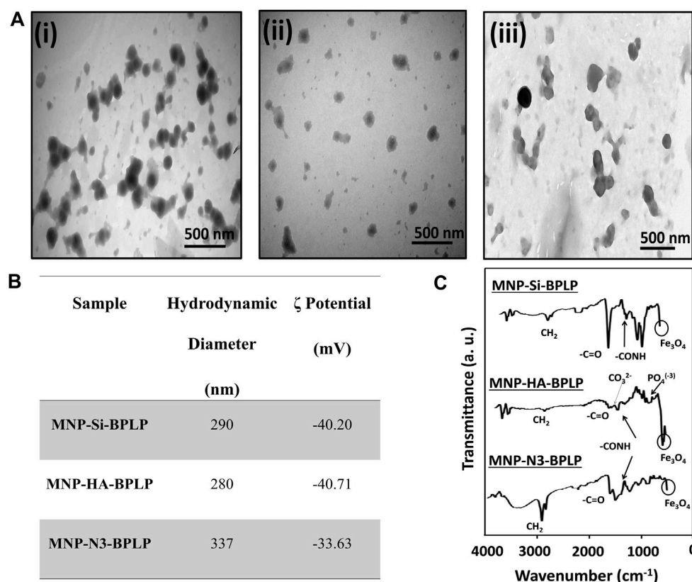
FIGURE 2 Physicochemical characterization of mDICT-NPs. (A) TEM images showing the core-shell structures of NPs: (i) MNP-Si-BPLP (ii) MNP-HA-BPLP (iii) MNP-N 3 -BPLP. (B) Hydrodynamic diameters and zeta potentials (ζ) of MNP-Si-BPLP, MNP-HA-BPLP and MNP-N 3 -BPLP. (C) FTIR spectra of MNP-Si-BPLP, MNP-HA-BPLP and MNP-N 3 -BPLP showing MNP and BPLP constituent chemical peaks.
